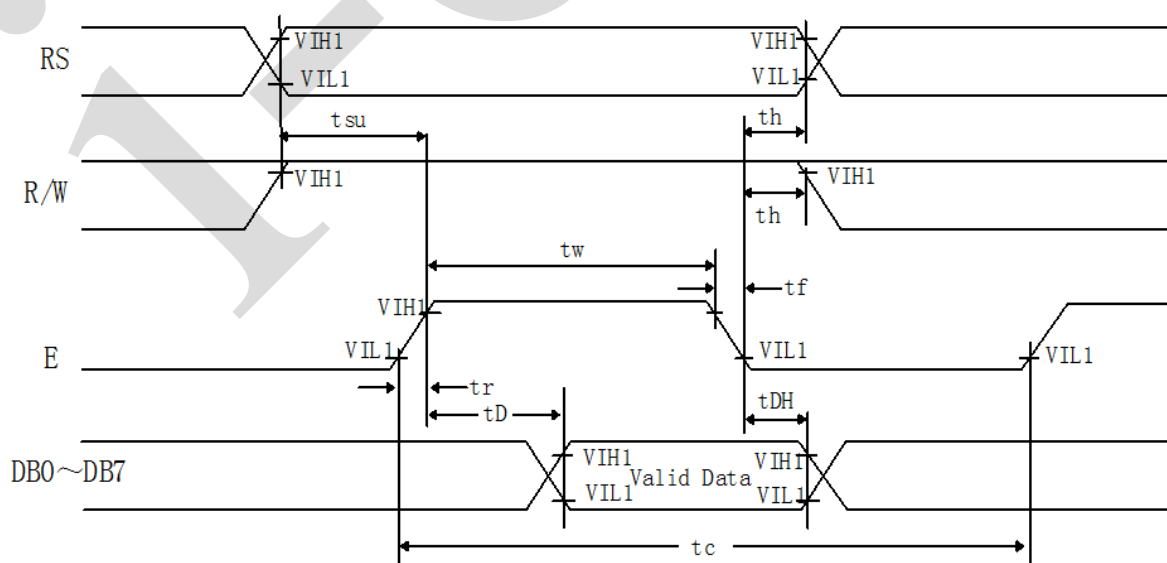
Figure 2 . Read Mode Timing Diagram
