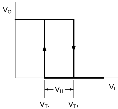
Figure 6. Transfer characteristic
