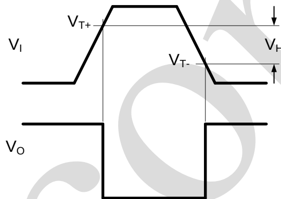
Figure 7. The definitions of V_{T+} , V_{T-} and V_H
