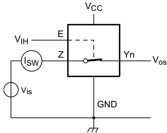
Figure 7. Test circuit for measuring ON-state leakage current
