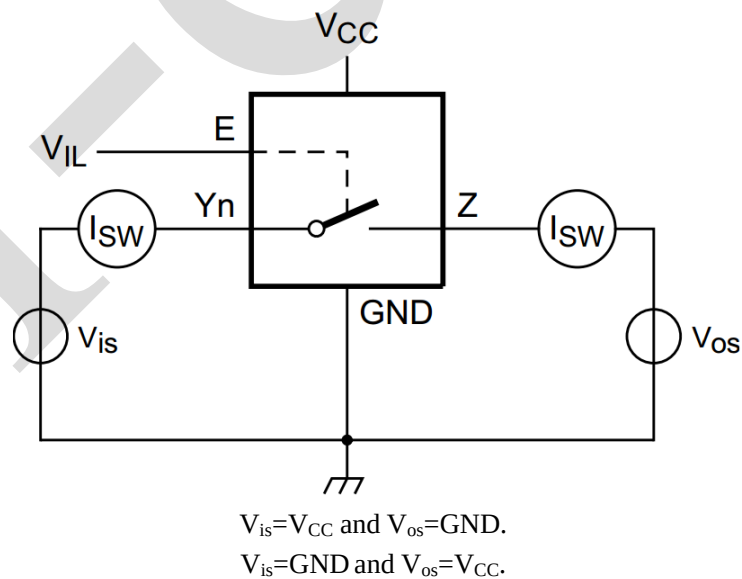
Figure 6. Test circuit for measuring OFF-state leakage current
