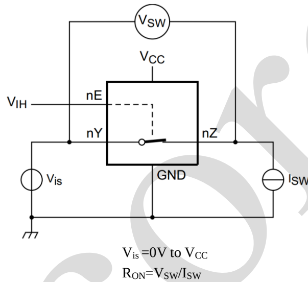
Figure 5. Test circuit for measuring R_{ON}
