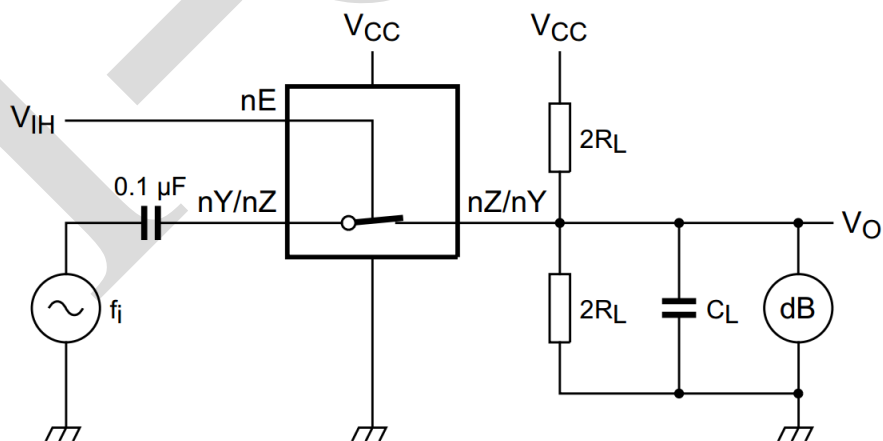
Figure 13. -3 dB frequency response
