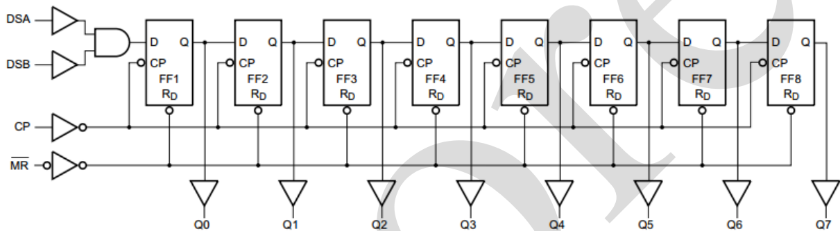
Figure 4. Functional diagram
