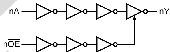
Figure 3. Logic diagram
