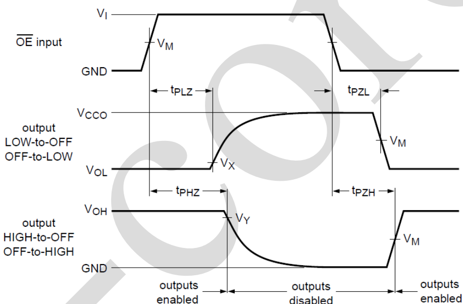
V_{OL} and V_{OH} are typical output voltage levels that occur with the output load.
