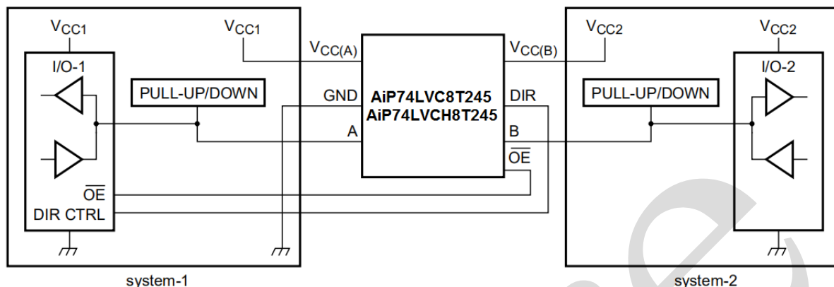
Figure 13. Bidirectional logic level-shifting application
